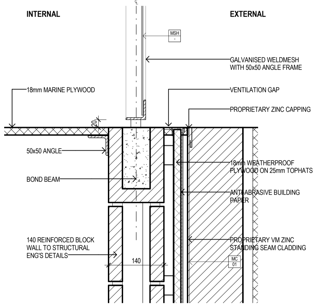
5 630_SECTION_TYPICAL ZINC CLADDING DETAILS (TOP) A501 1:5
