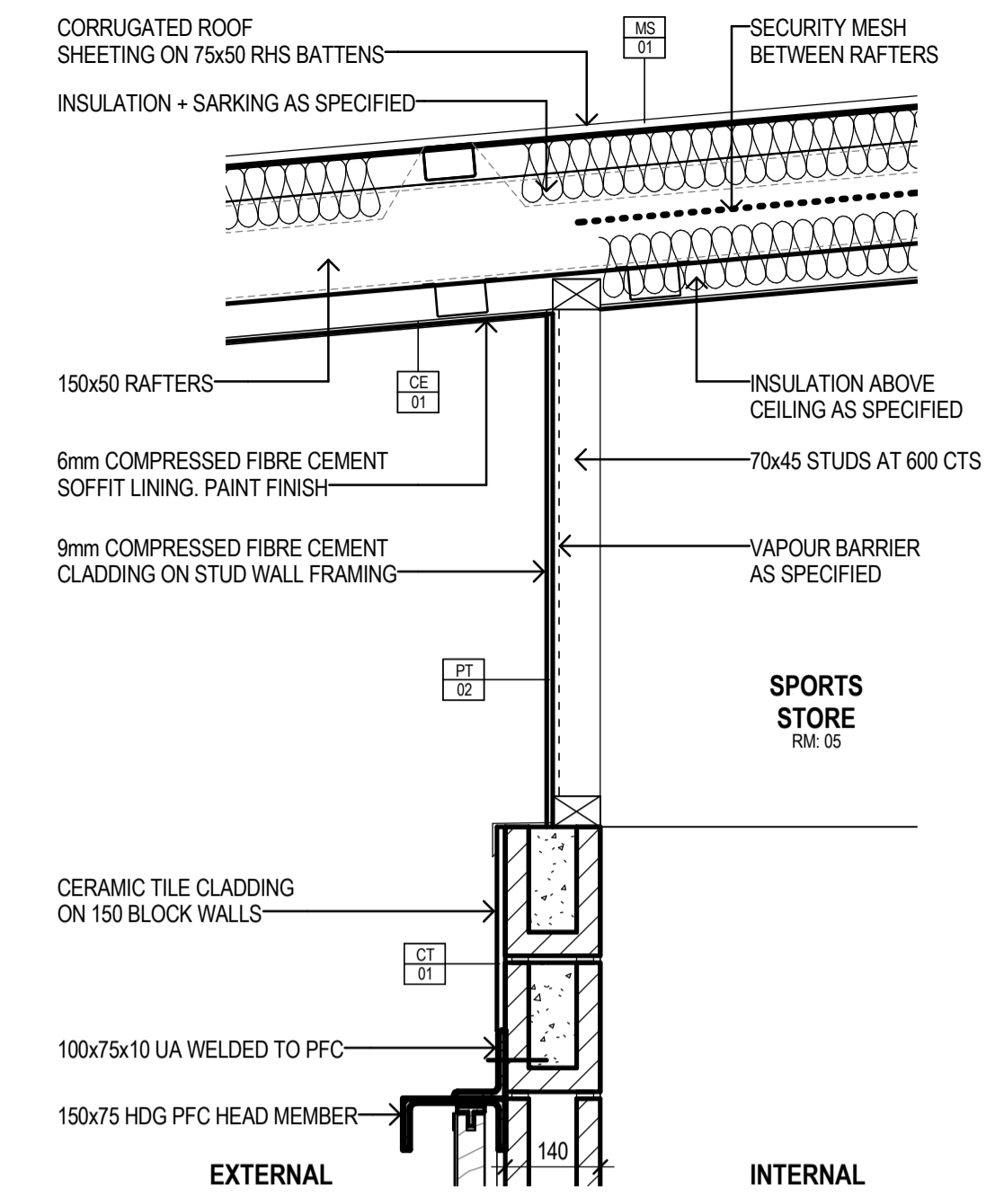
9 630_SECTION_TYPICAL DETAIL FC SPANDEL A501 1:10
