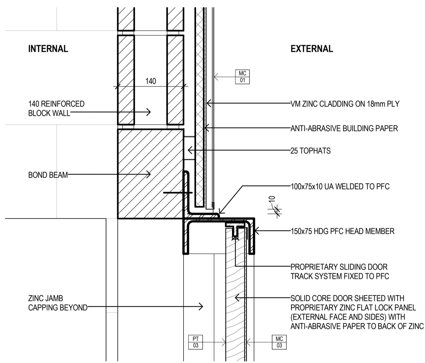
2 630_SECTION_TYPICAL SLIDING DOOR HEAD DETAIL A501 1:5
