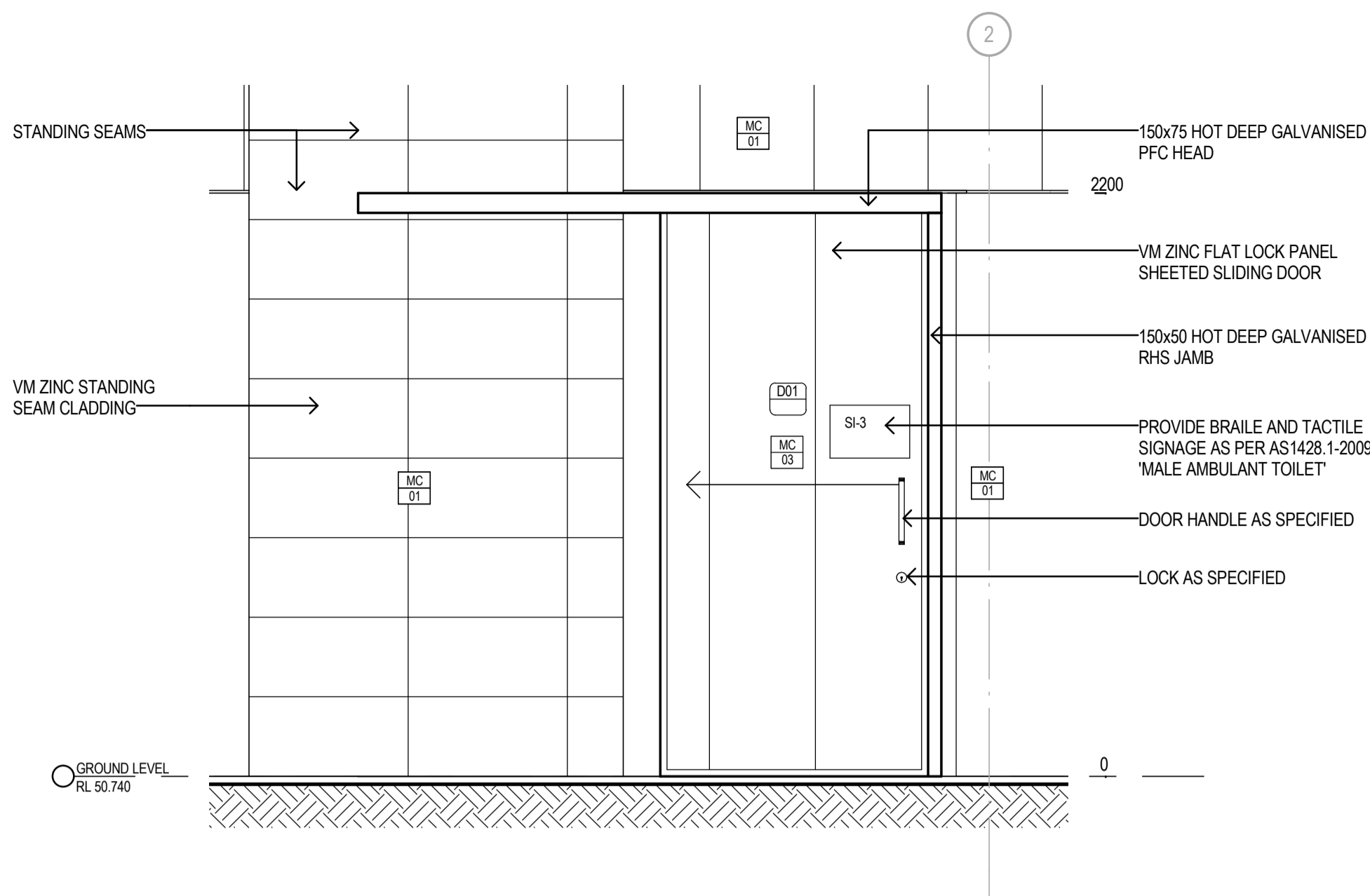
1 360_ELEVATION_TYPICAL SLIDING DOOR A401 1:20
