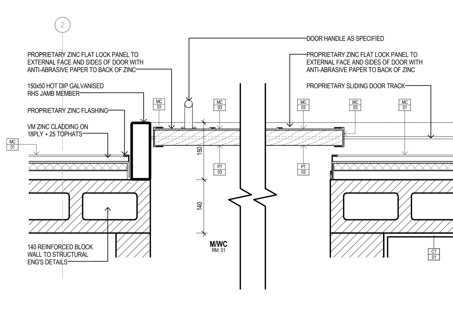
4 630_PLAN_TYPICAL SLIDING DOOR JAMB DETAILS A801 1:5
