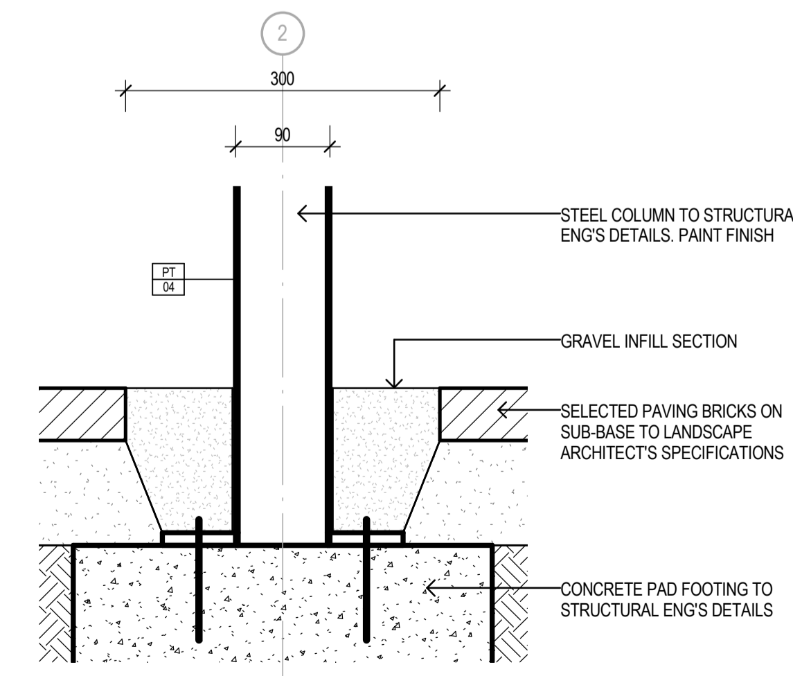
8 630_SECTION_EXTERNAL COLUMN BASE DETAIL A632 1:5
