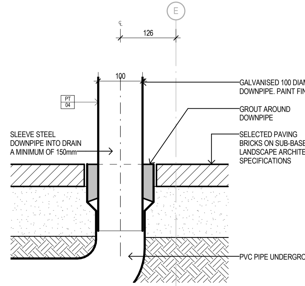
11 630_SECTION_TYPICAL DOWNPIPE BOTTOM DETAIL A501 1:5
