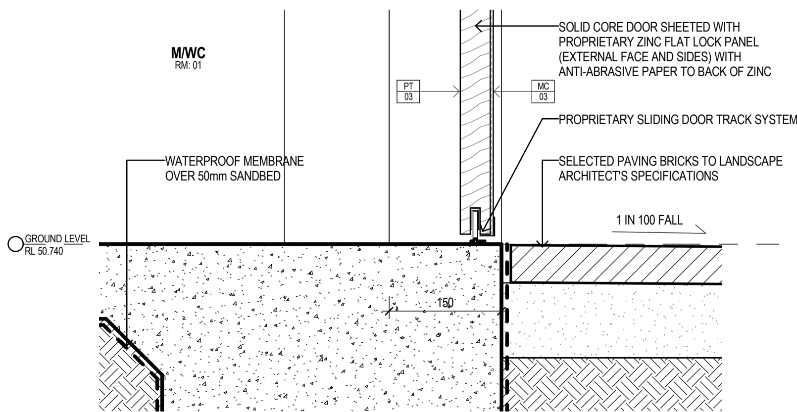
3 630_SECTION_TYPICAL SLIDING DOOR BOTTOM DETAIL A501 1:5
