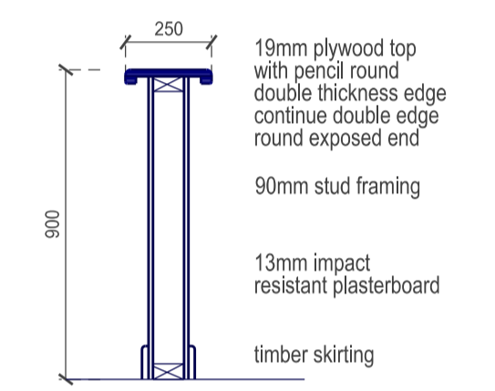
PLAYROOM 1 LOW WALL 1:20
