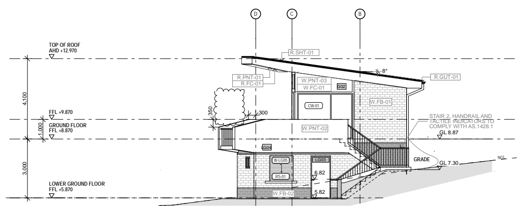
2 NORTH ELEVATION 1:100
