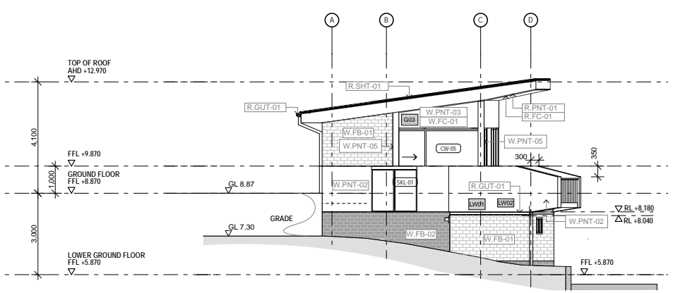
2 SOUTH ELEVATION 1:100
