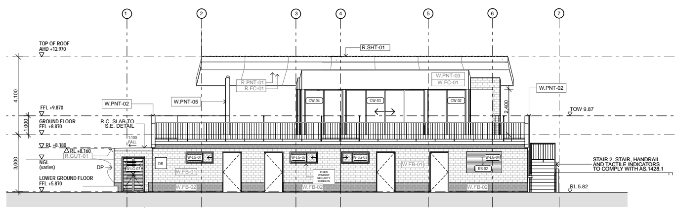
4 EAST ELEVATION 1:100
