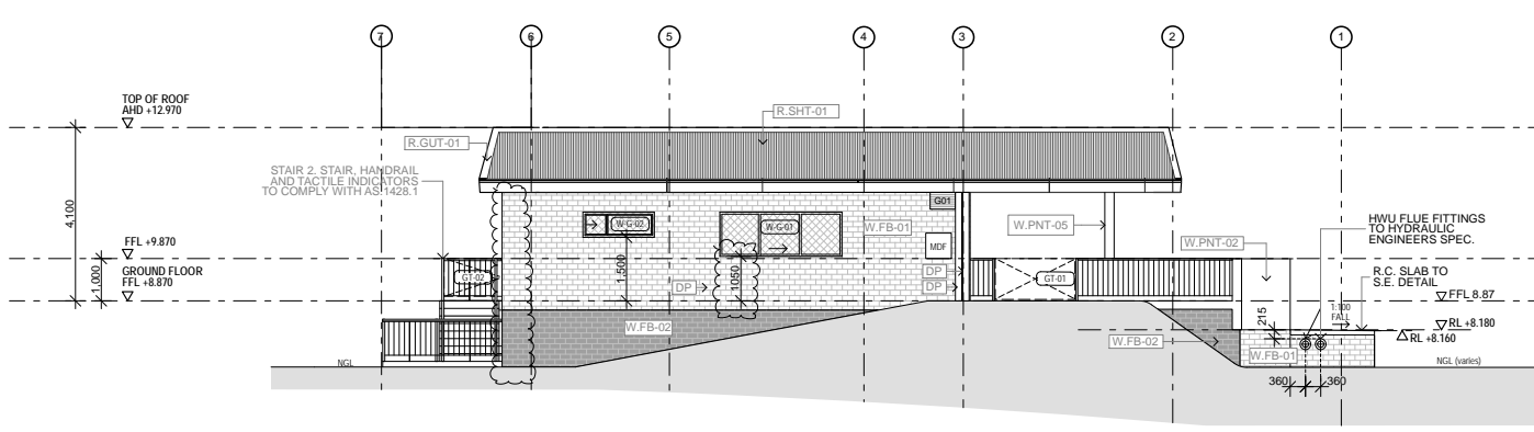
3 WEST ELEVATION 1:100
