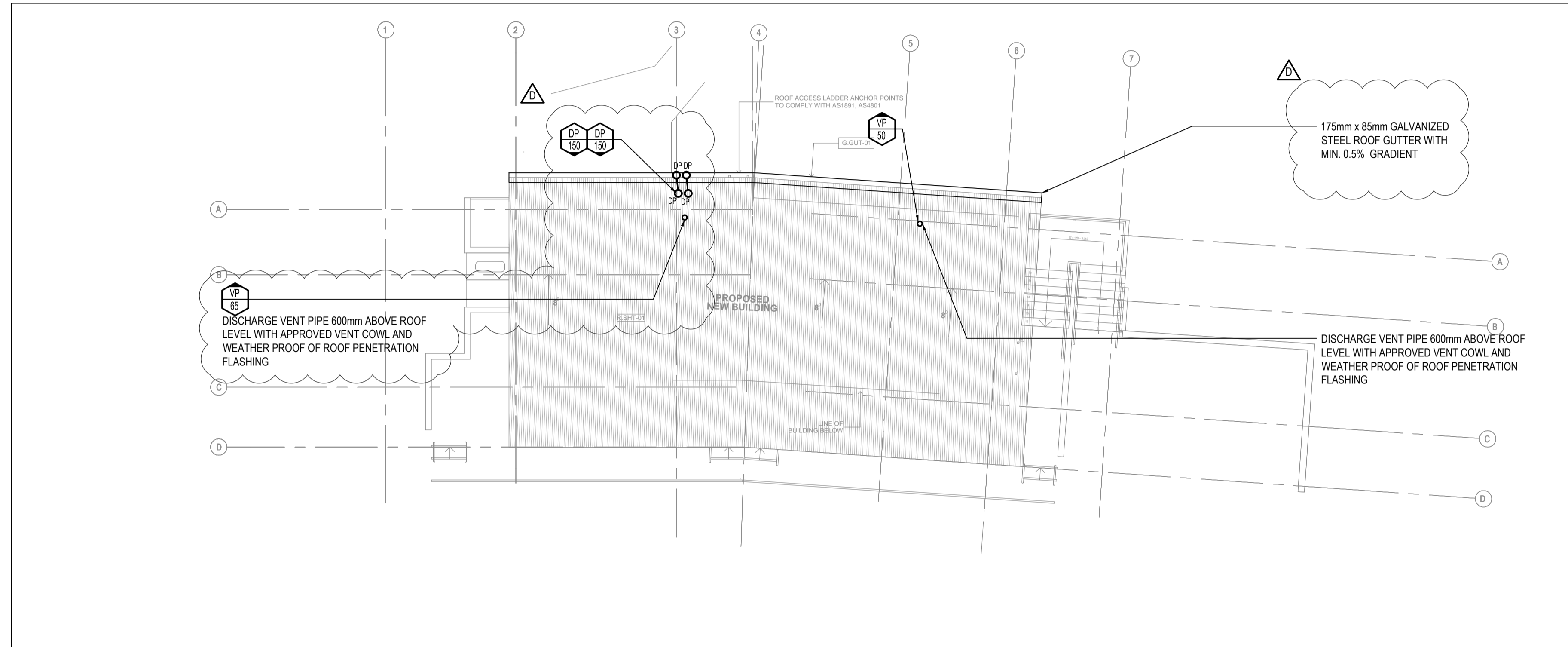
ROOF - STORMWATER LAYOUT SCALE 1:100
