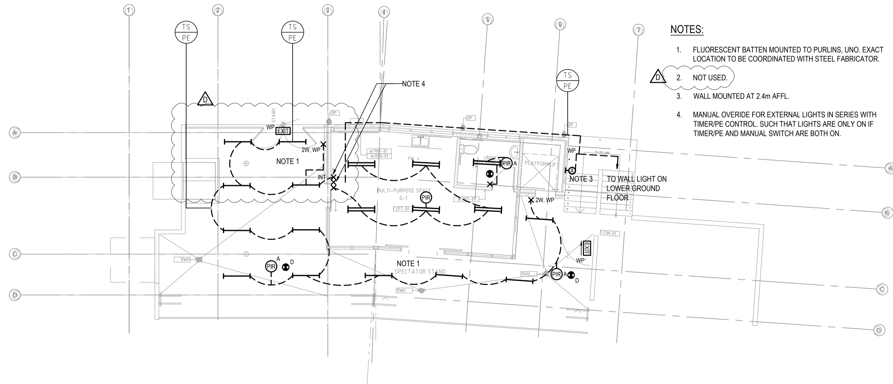
LOWER GROUND FLOOR - LIGHTING LAYOUT SCALE 1:100
